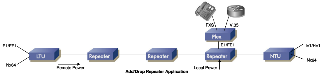
Add/Drop Repeater Application
