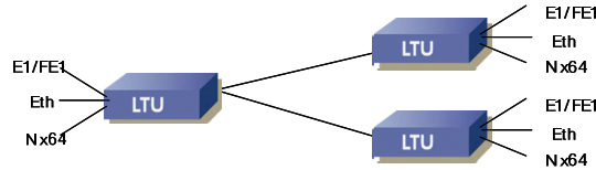
Point to Multipoint Application
